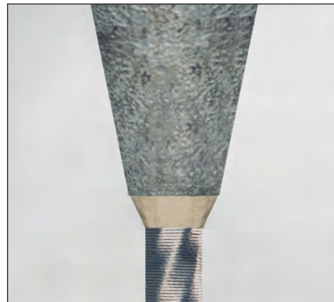
Axes of socket and rope properly aligned and sealed with plasticine (Fig. 4)
