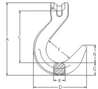
A-1359 Clevis Foundry Hook
