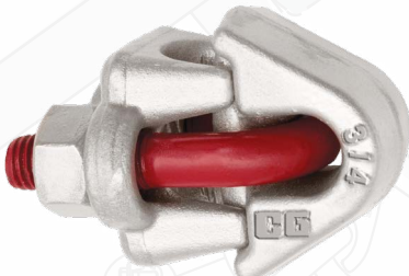
G-461 "Thimble Eye" Bundle Clip
