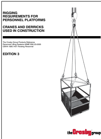
Personnel Platform
